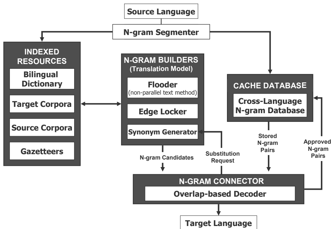
Figure 1. CBMT Basic Run-Time Architecture
