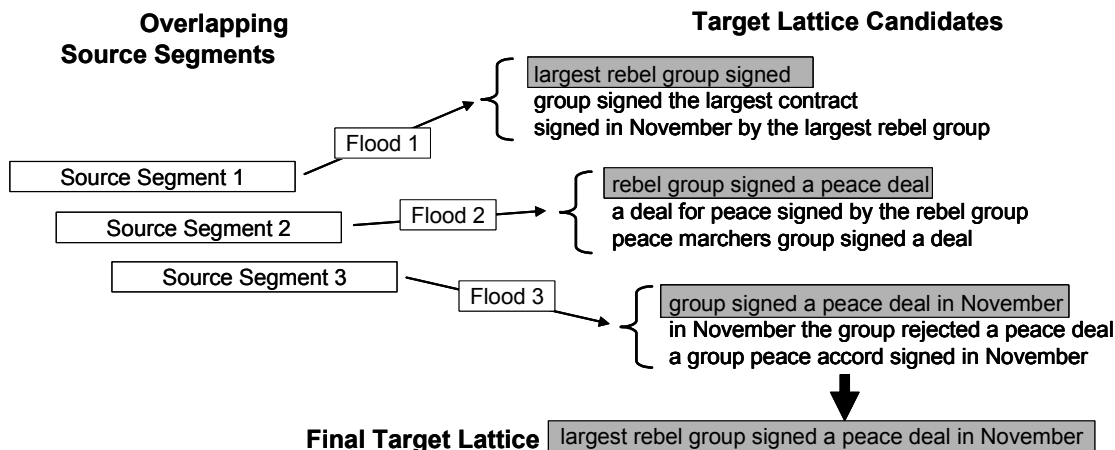
Figure 2. Lattice Overlap
